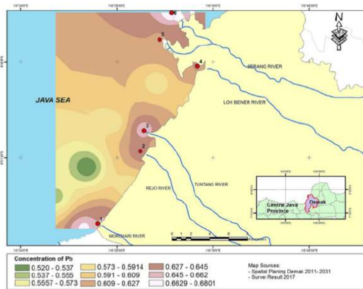
Fig. 2. The distribution of Pb ( \text{mg}\cdot\text{l}^{-1} ) in Demak waters
