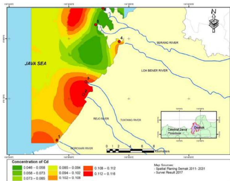
Fig. 3. The distribution of Cadmium ( \text{mg}\cdot\text{l}^{-1} ) in Demak waters
