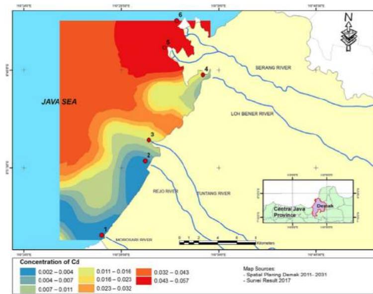
Fig. 5. Cd content in surface sediment ( \text{mg}\cdot\text{l}^{-1} ) in Demak waters
