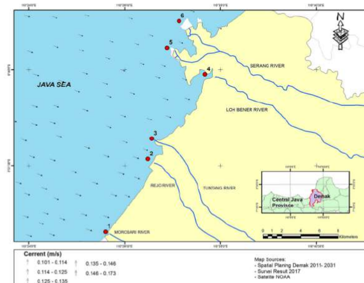
Fig. 7. Currents in Demak waters
