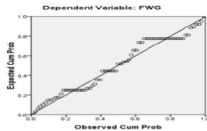
Figure 1. Normality Test result
